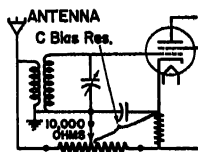
Antenna C-bias volume-control circuit.
